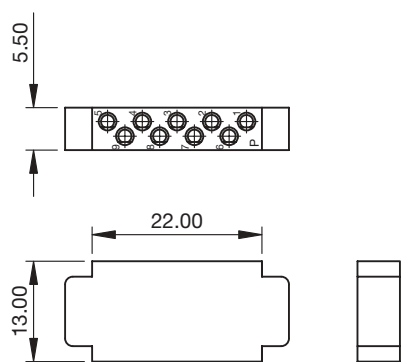
INSULATING BLOCK: Ref. QHP
