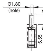
Ref. XRf (AWG 16-20) (contacts are supplied not assembled)
